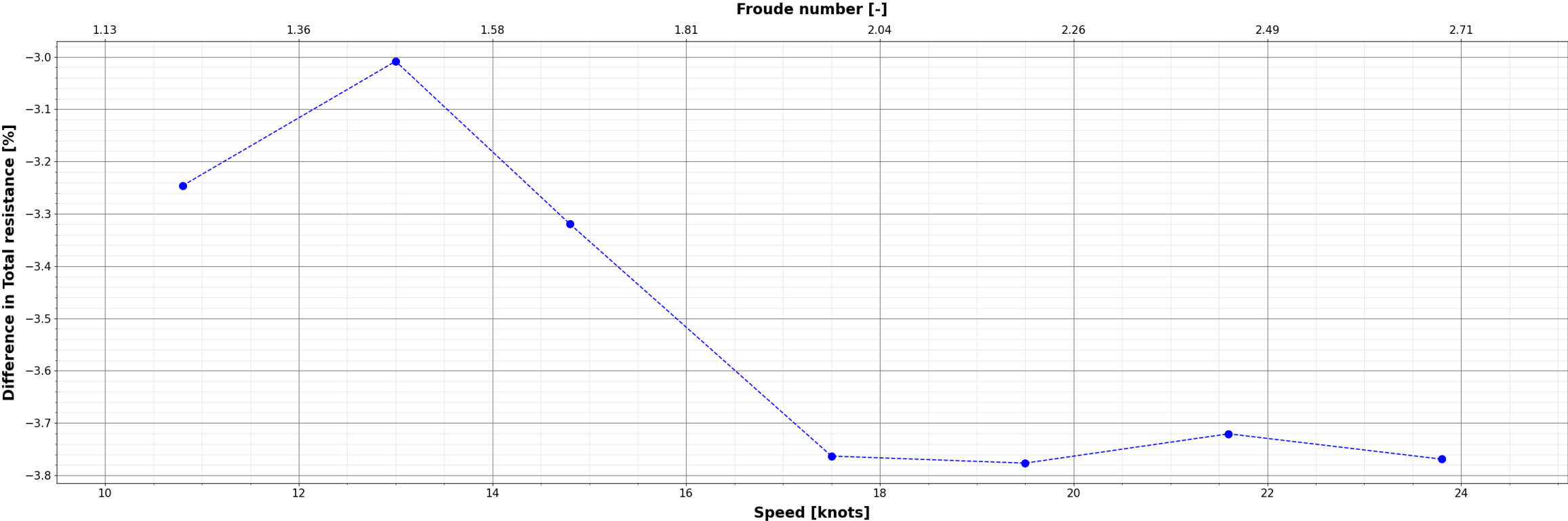
Comparison of Total resistance : (X_{\{i\}} - GPPH\_EFD) / GPPH\_EFD
