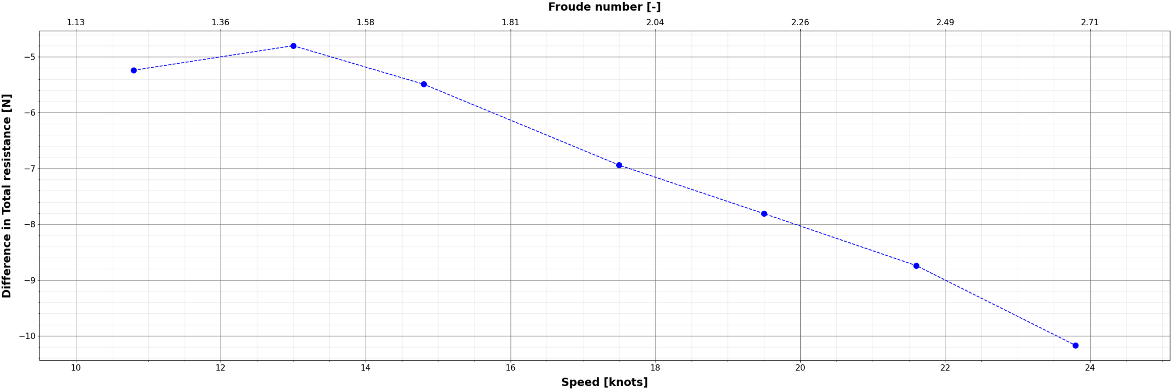
Comparison of Total resistance : X_{\{i\}} - GPPH_EFD
