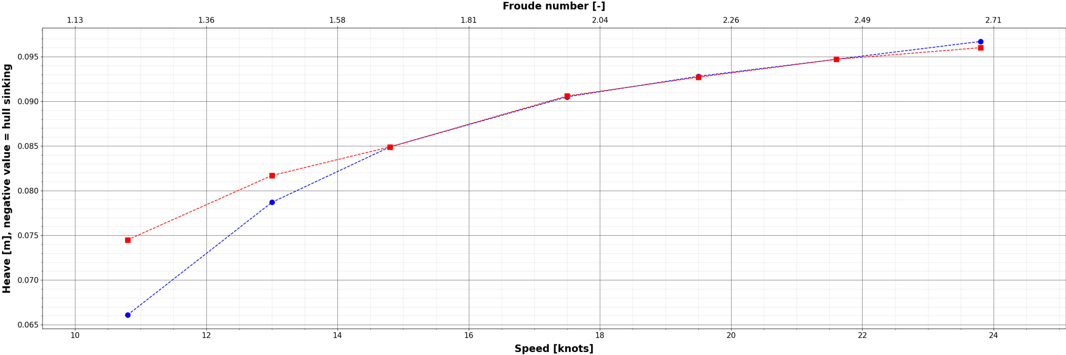
Evolution of dynamic heave attitude
