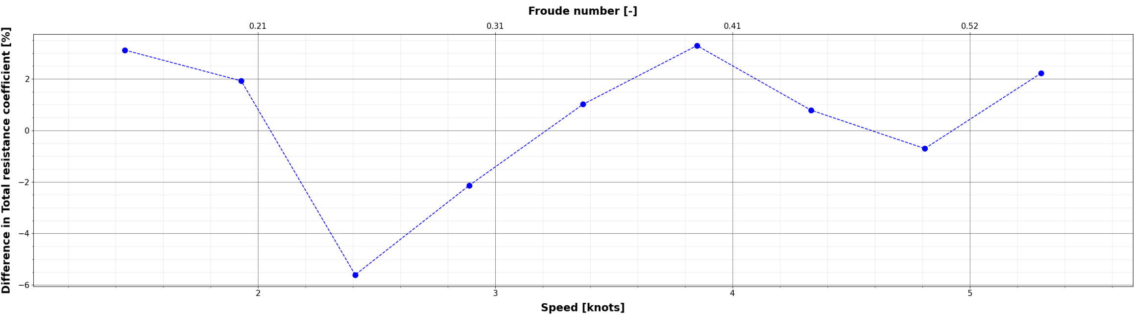
Comparison of Total resistance coefficient : (X_{\{i\}} - S60\_Mono\_EFD) / S60\_Mono\_EFD
