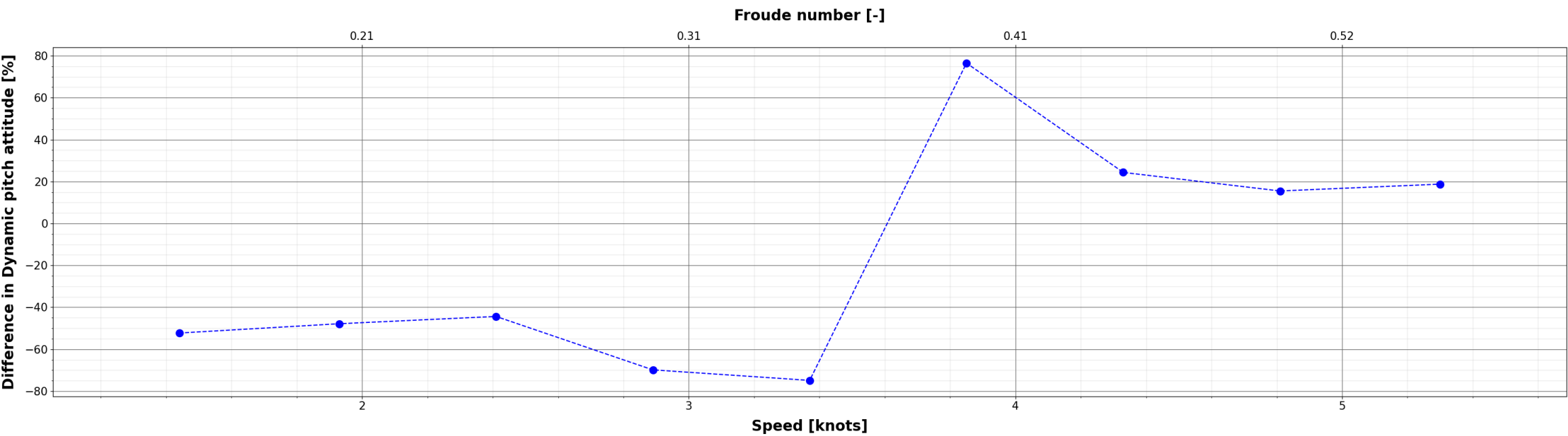
Comparison of Dynamic pitch attitude : (X_{\{i\}} - S60\_Mono\_EFD) / S60\_Mono\_EFD
