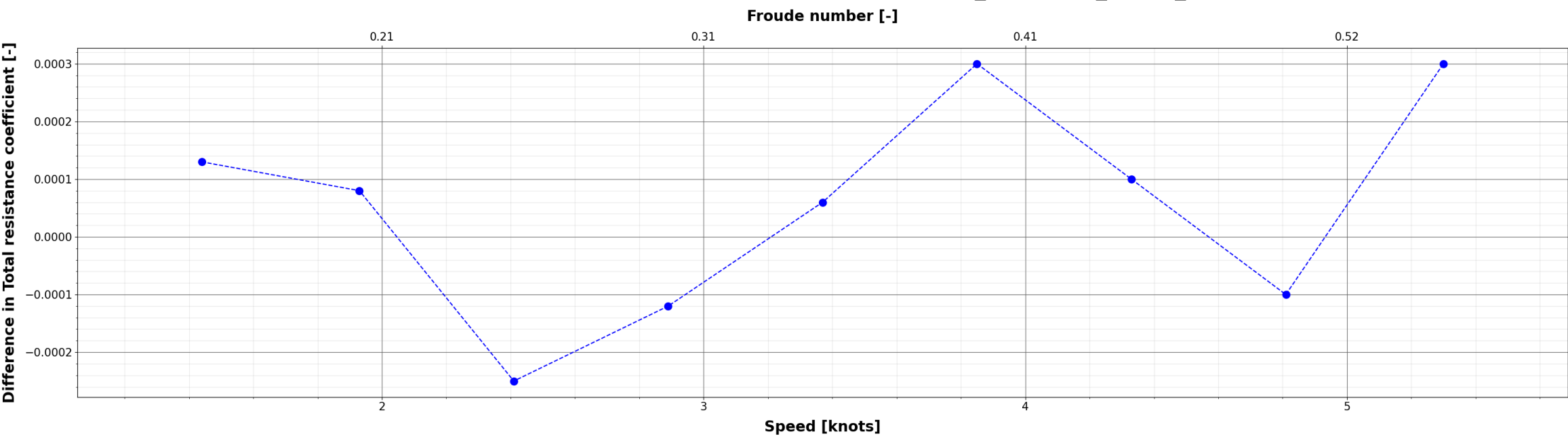
Comparison of Total resistance coefficient : X_{\{i\}} - S60_Mono_EFD
