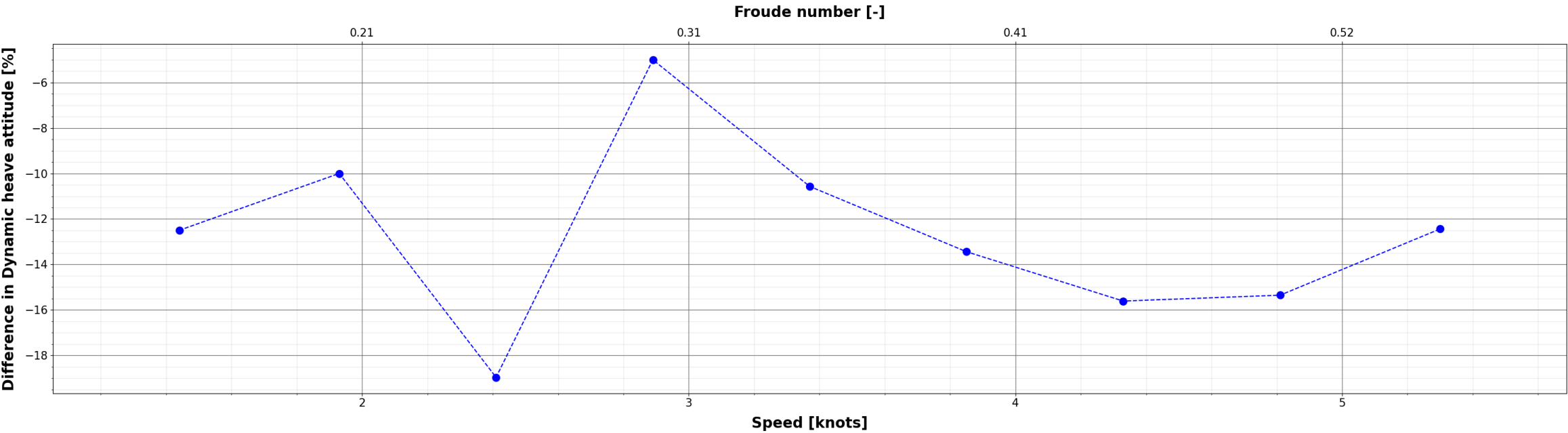
Comparison of Dynamic heave attitude : (X_{\{i\}} - S60\_Mono\_EFD) / S60\_Mono\_EFD
