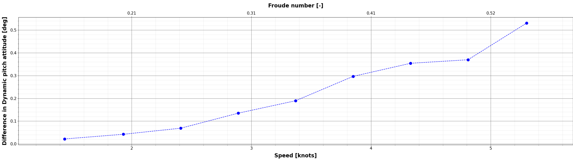
Comparison of Dynamic pitch attitude : X_{\{i\}} - S60_Mono_EFD
