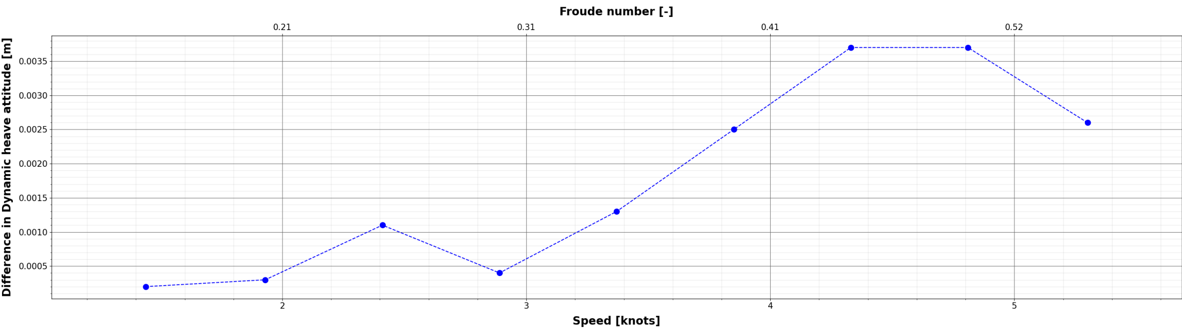
Comparison of Dynamic heave attitude : X_{\{i\}} - S60_Mono_EFD
