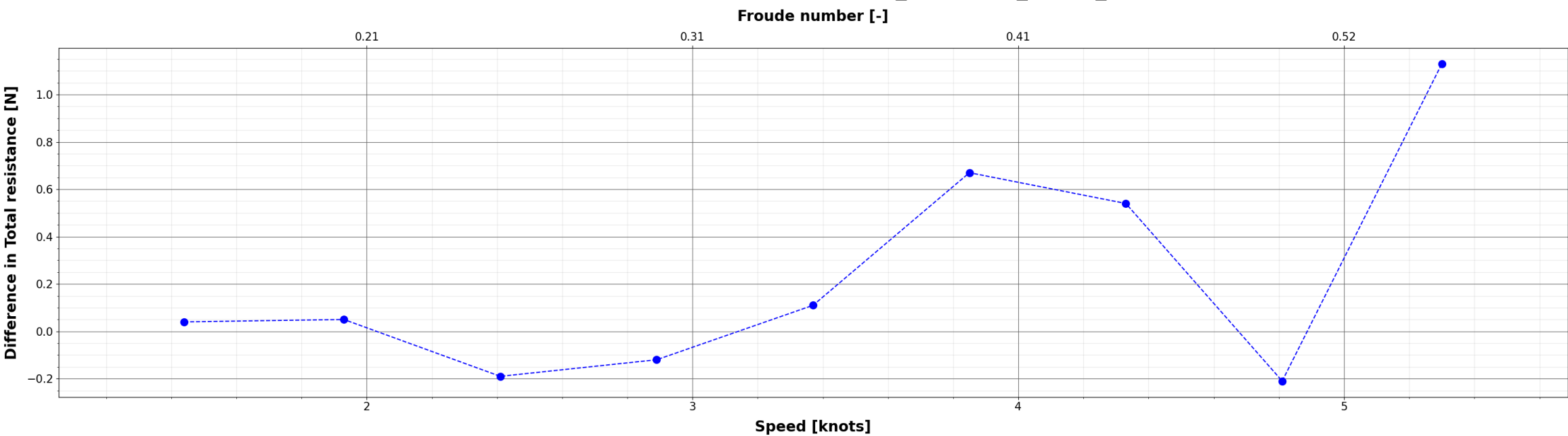
Comparison of Total resistance : X_{\{i\}} - S60_Mono_EFD
