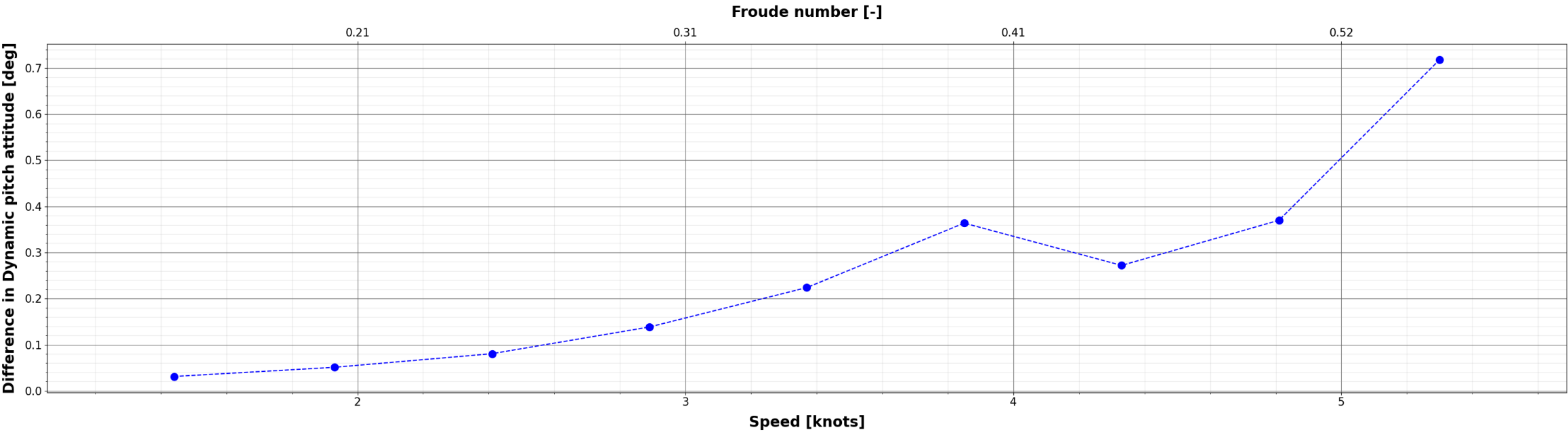
Comparison of Dynamic pitch attitude : X_{\{i\}} - S60_S1174_EFD
