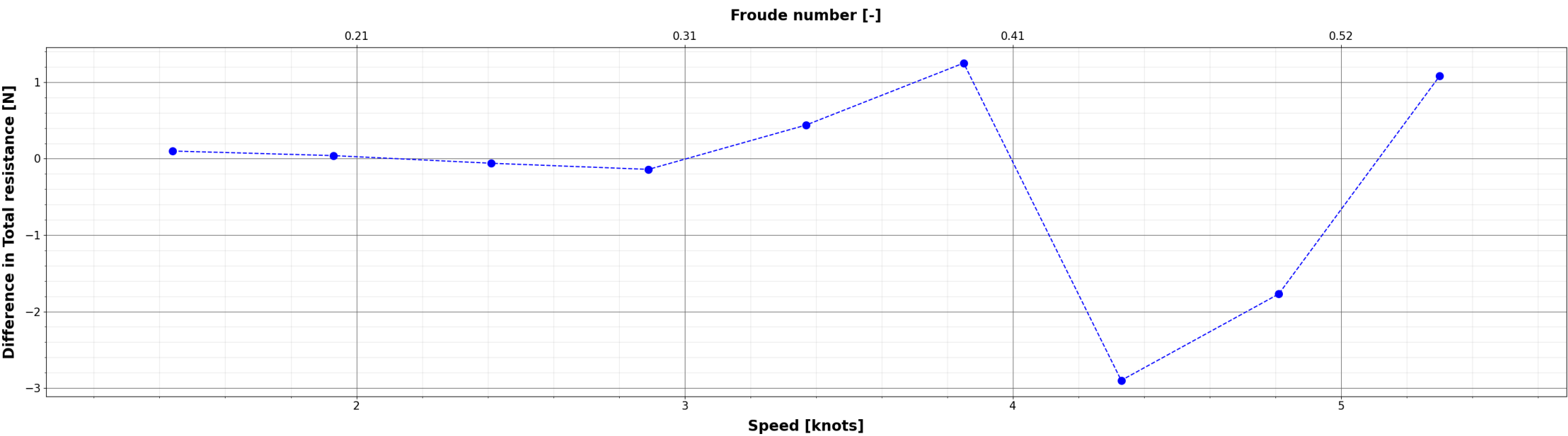
Comparison of Total resistance : X_{\{i\}} - S60_S1174_EFD
