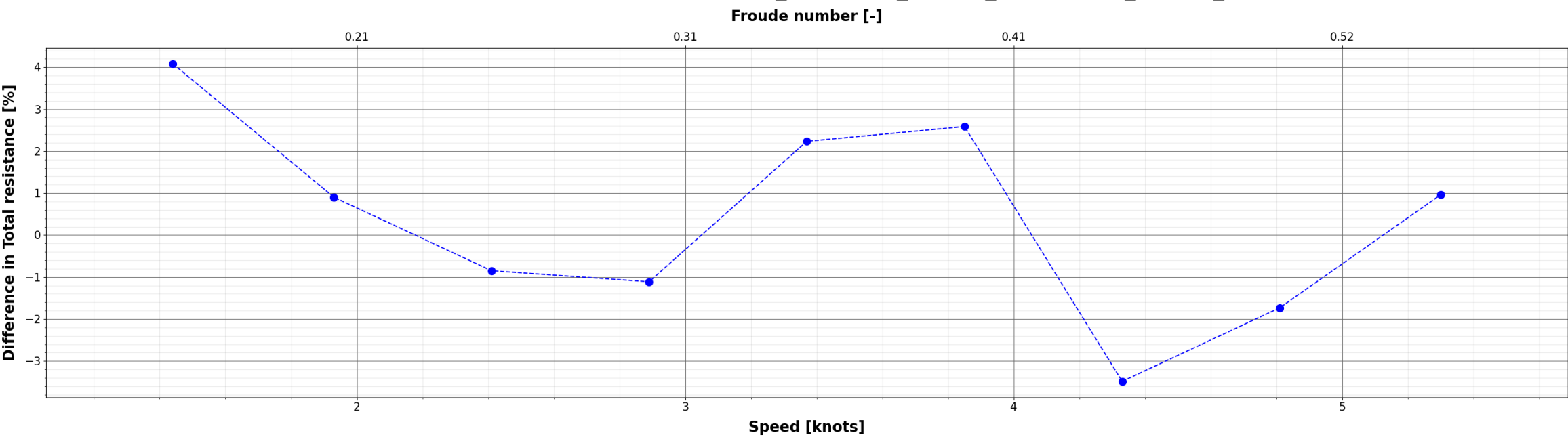
Comparison of Total resistance : (X_{\{i\}} - S60\_S1174\_EFD) / S60\_S1174\_EFD
