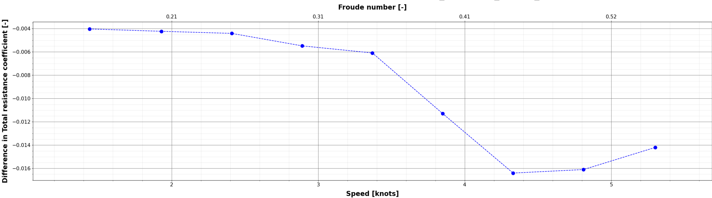
Comparison of Total resistance coefficient : X_{\{i\}} - S60_S1174_EFD
