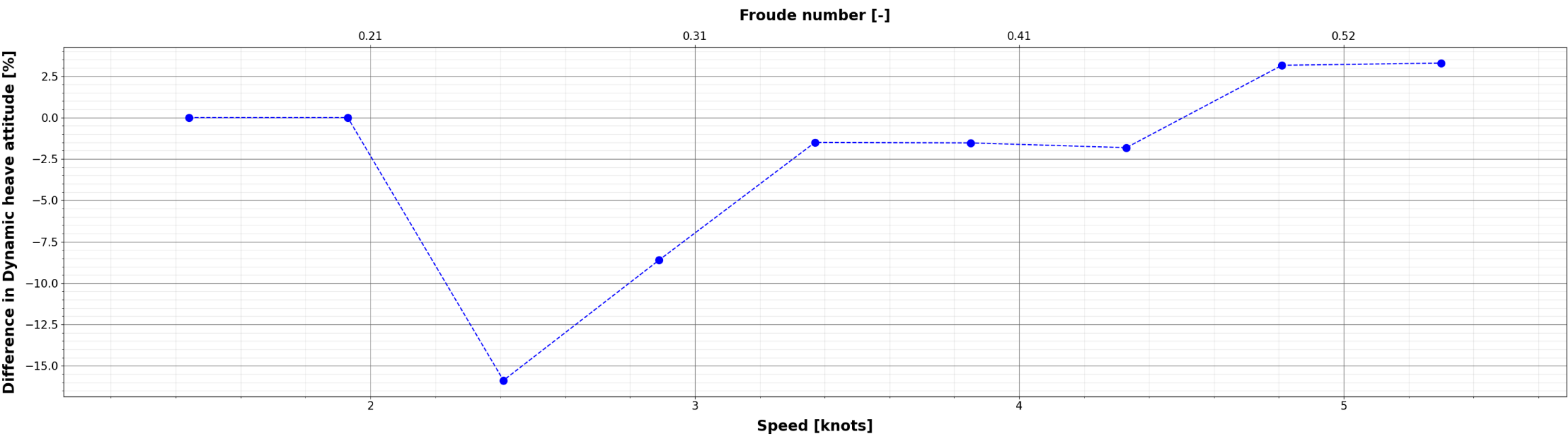
Comparison of Dynamic heave attitude : (X_{\{i\}} - S60\_S1174\_EFD) / S60\_S1174\_EFD
