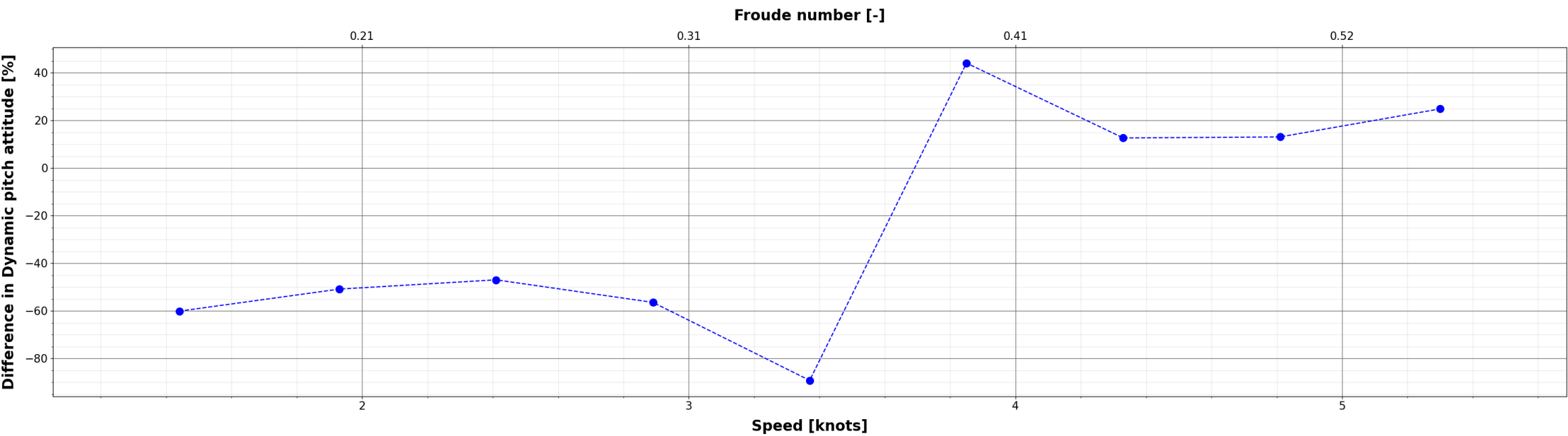
Comparison of Dynamic pitch attitude : (X_{\{i\}} - S60\_S1174\_EFD) / S60\_S1174\_EFD
