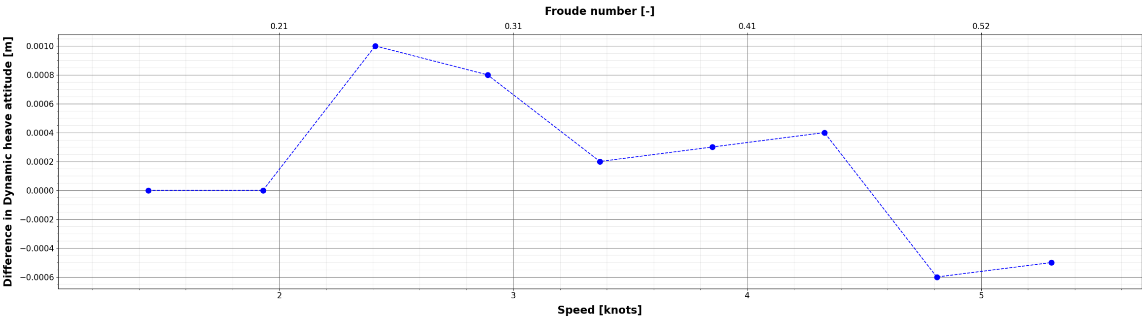
Comparison of Dynamic heave attitude : X_{\{i\}} - S60_S1174_EFD
