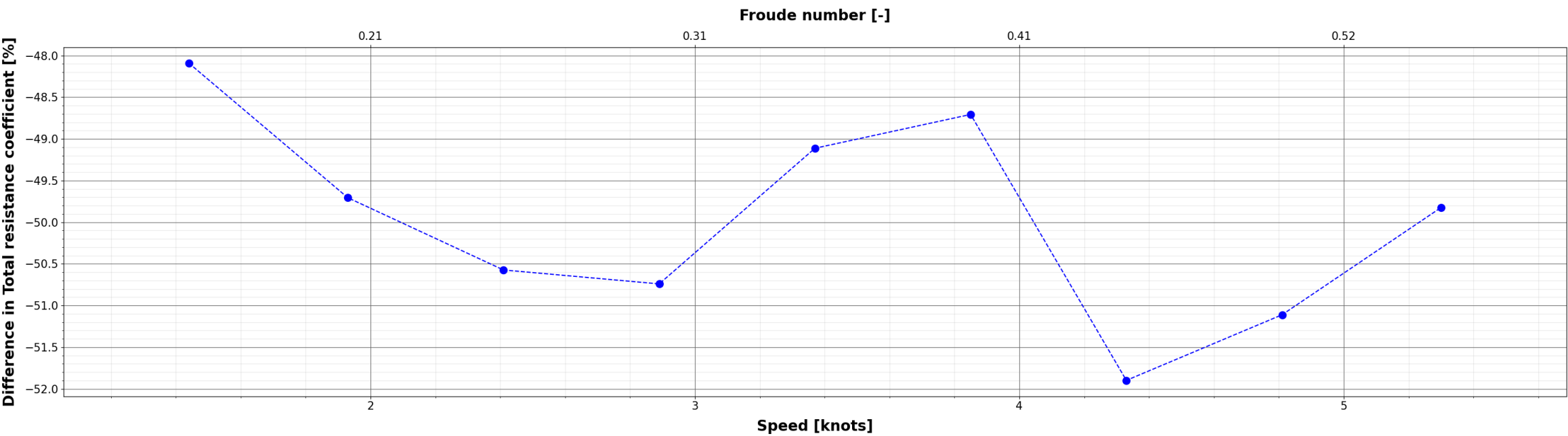
Comparison of Total resistance coefficient : (X_{\{i\}} - S60\_S1174\_EFD) / S60\_S1174\_EFD
