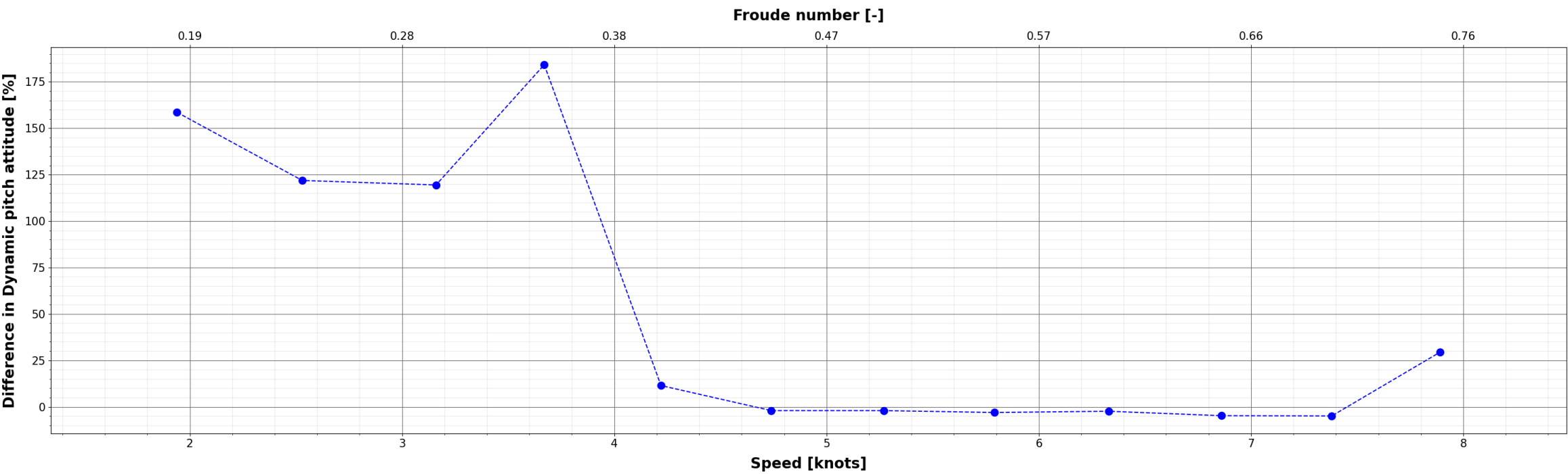
Comparison of Dynamic pitch attitude : (X_{\{i\}} - \text{DELFT\_372\_EFD}) / \text{DELFT\_372\_EFD}
