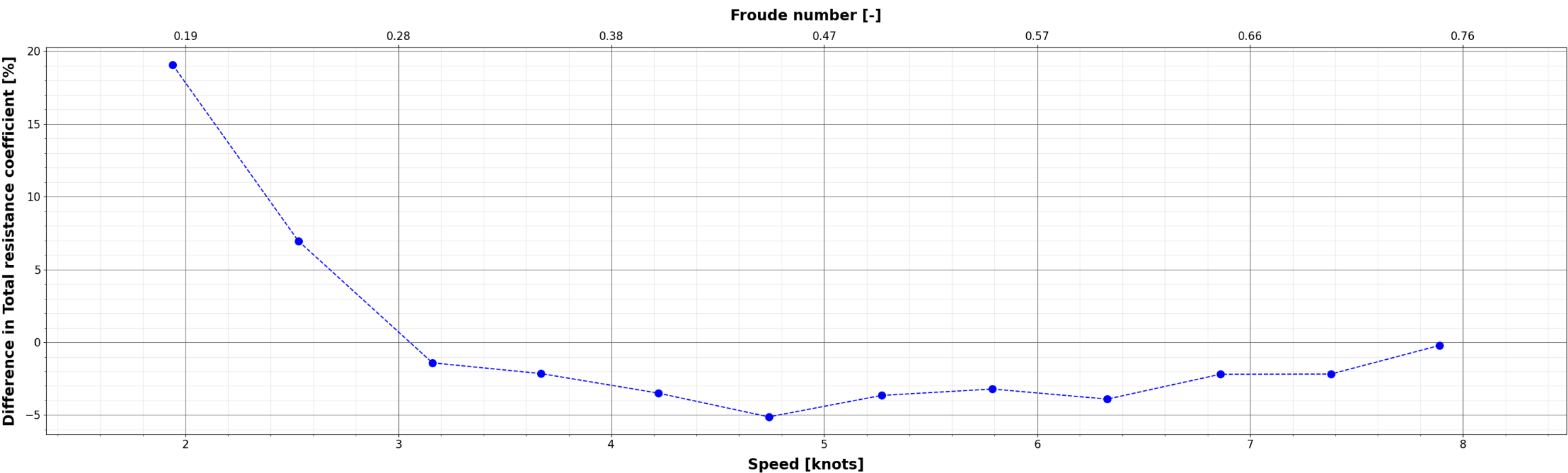
Comparison of Total resistance coefficient : (X_{\{i\}} - \text{DELFT\_372\_EFD}) / \text{DELFT\_372\_EFD}
