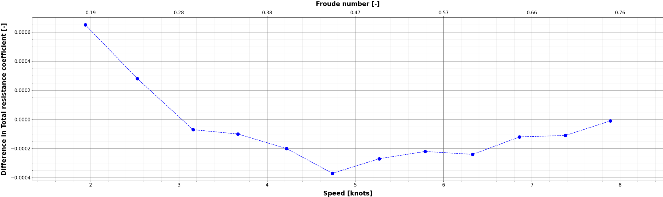
Comparison of Total resistance coefficient : X_{\{i\}} - DELFT_372_EFD
