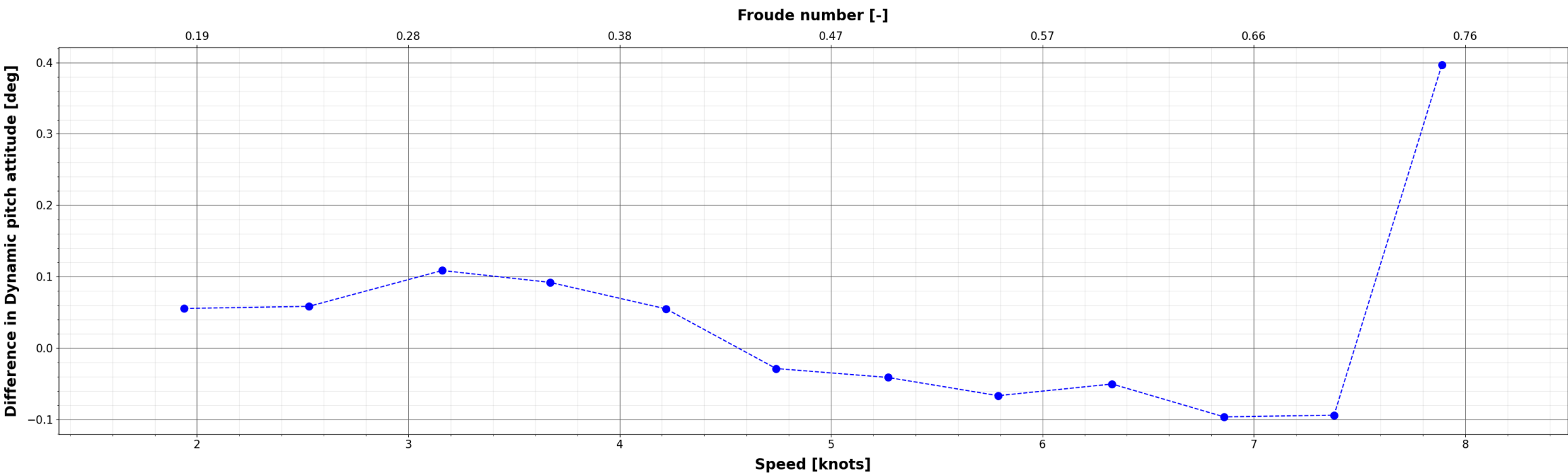
Comparison of Dynamic pitch attitude : X_{\{i\}} - DELFT_372_EFD
