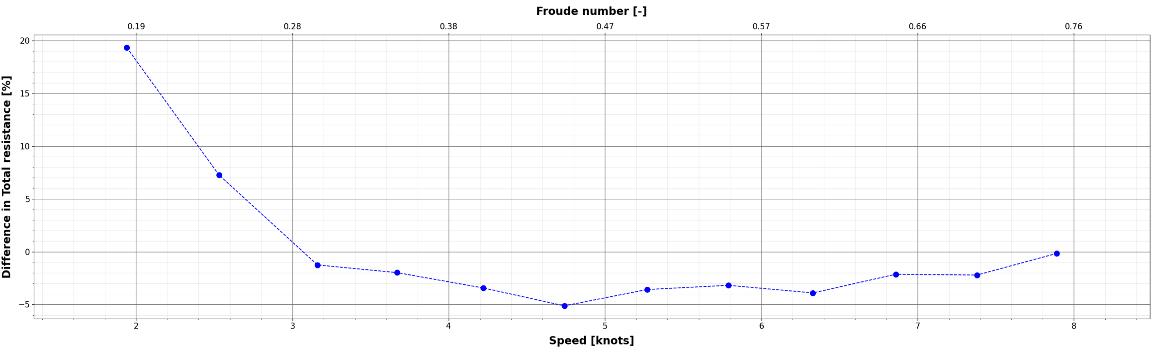
Comparison of Total resistance : (X_{\{i\}} - \text{DELFT\_372\_EFD}) / \text{DELFT\_372\_EFD}
