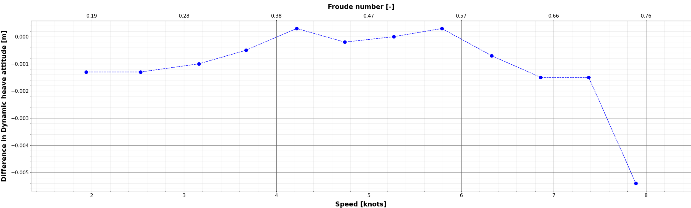
Comparison of Dynamic heave attitude : X_{\{i\}} - DELFT_372_EFD
