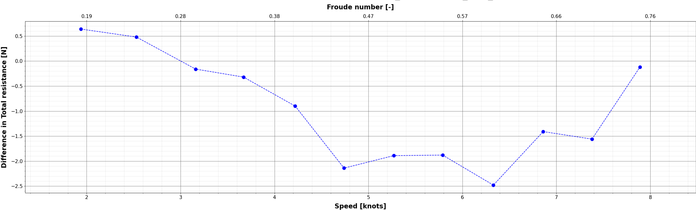
Comparison of Total resistance : X_{\{i\}} - DELFT_372_EFD
