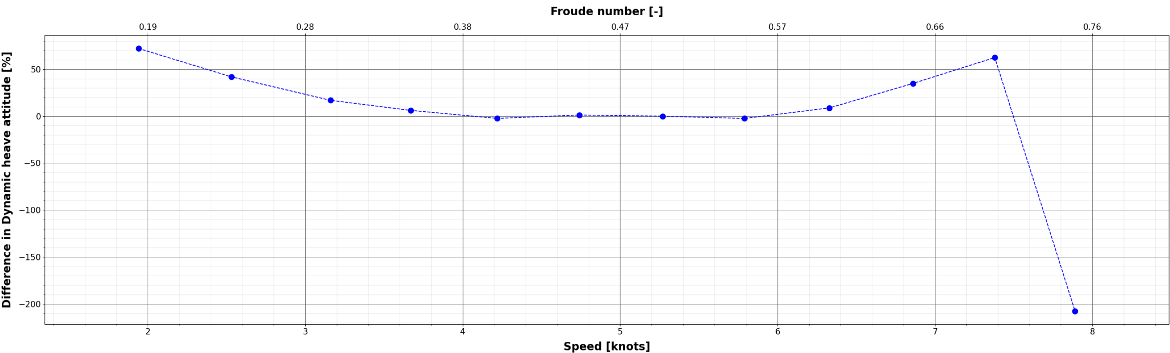
Comparison of Dynamic heave attitude : (X_{\{i\}} - \text{DELFT\_372\_EFD}) / \text{DELFT\_372\_EFD}
