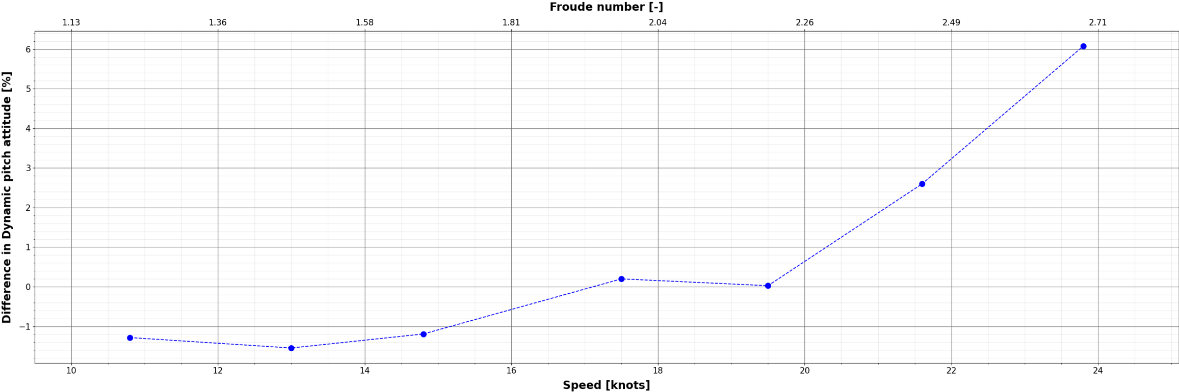
Comparison of Dynamic pitch attitude : (X_{\{i\}} - GPPH\_EFD) / GPPH\_EFD
