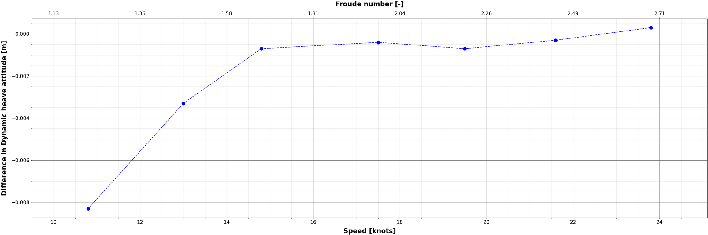
Comparison of Dynamic heave attitude : X_{\{i\}} - GPPH_EFD
