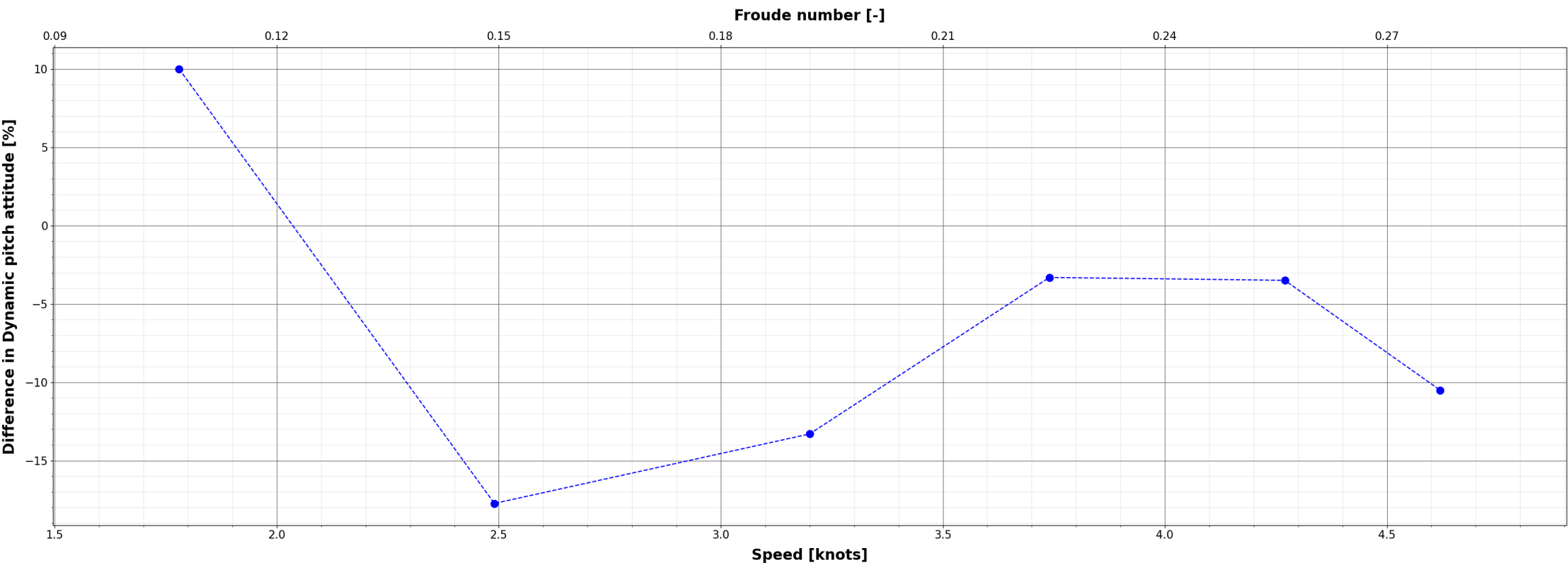
Comparison of Dynamic pitch attitude : (X_{\{i\}} - KCS\_EFD) / KCS\_EFD
