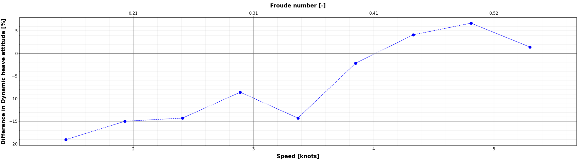
Comparison of Dynamic heave attitude : (X_{\{i\}} - S60\_S768\_EFD) / S60\_S768\_EFD
