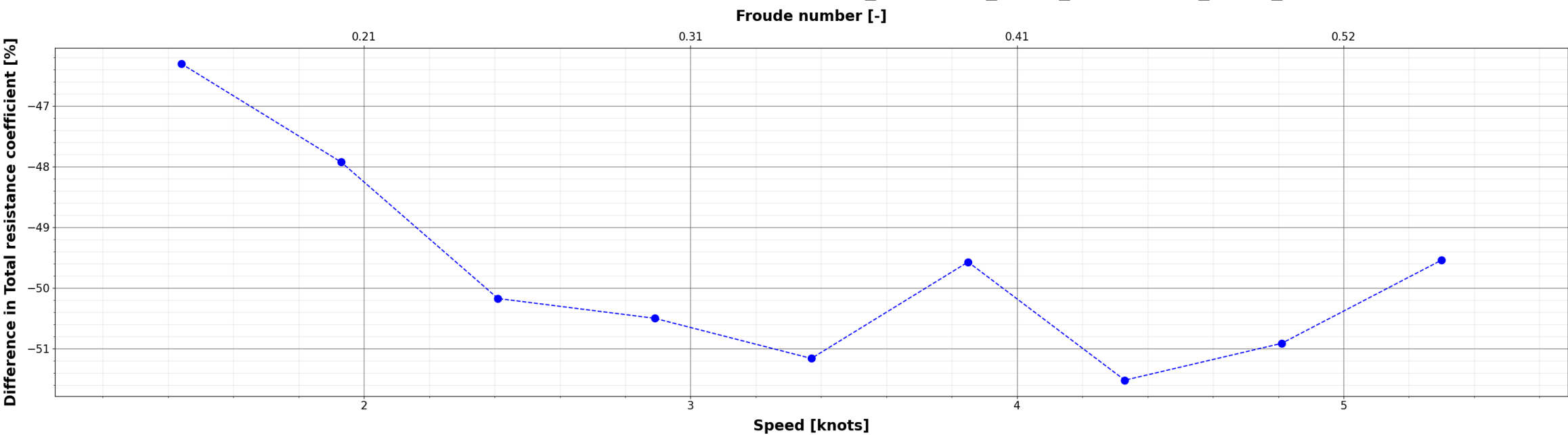
Comparison of Total resistance coefficient : (X_{\{i\}} - S60\_S768\_EFD) / S60\_S768\_EFD
