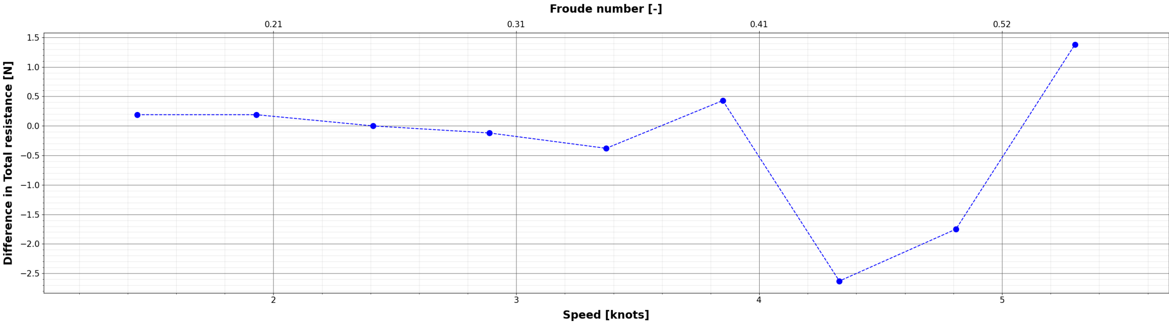
Comparison of Total resistance : X_{i} - S60_S768_EFD
