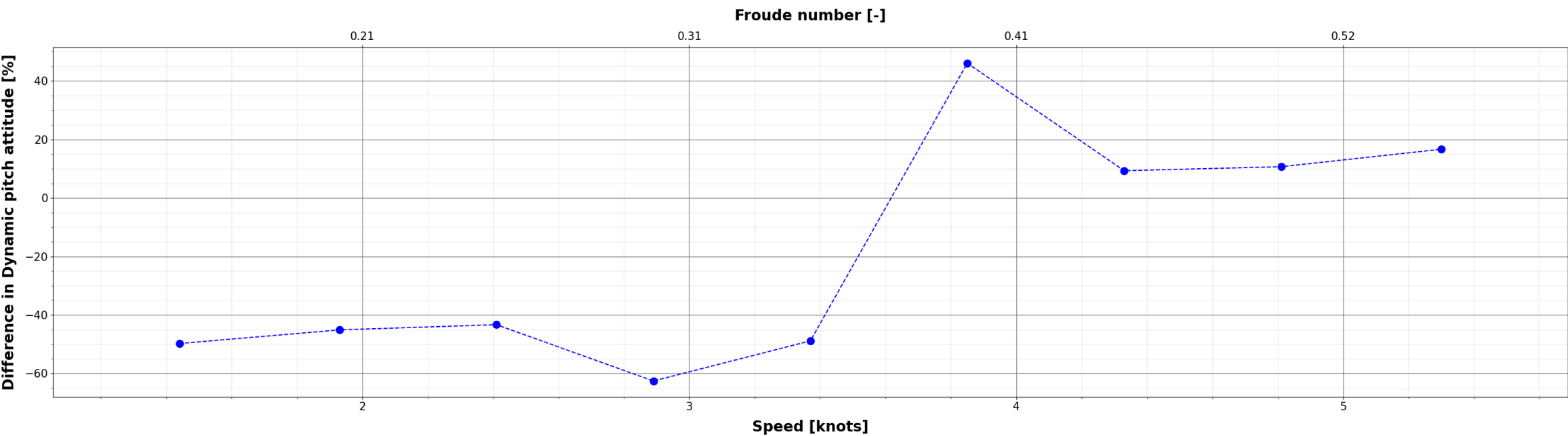
Comparison of Dynamic pitch attitude : (X_{\{i\}} - S60\_S768\_EFD) / S60\_S768\_EFD
