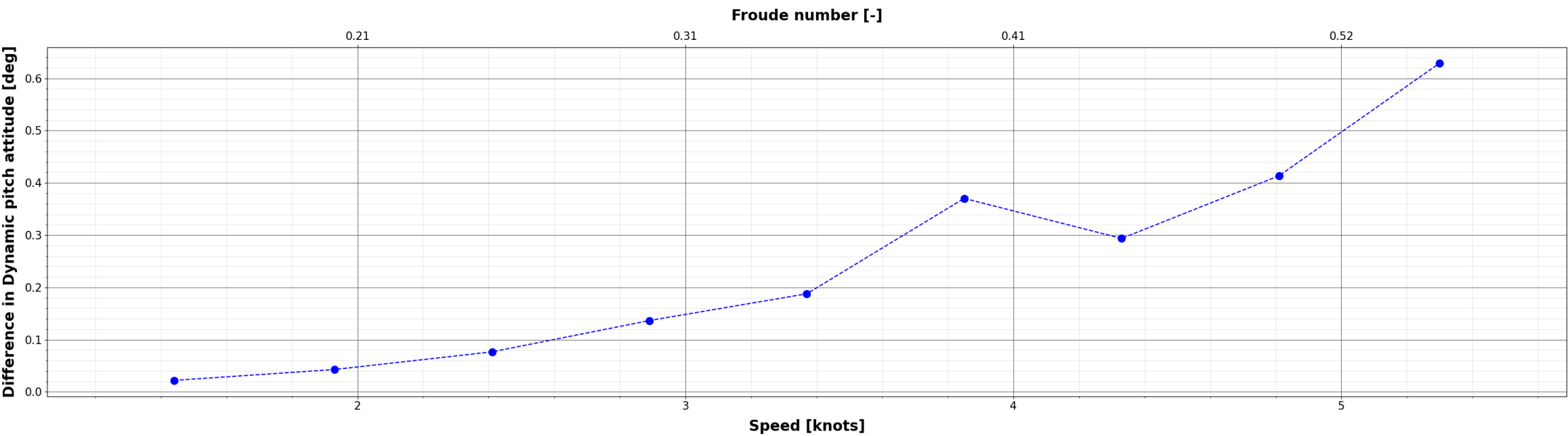
Comparison of Dynamic pitch attitude : X_{\{i\}} - S60_S768_EFD
