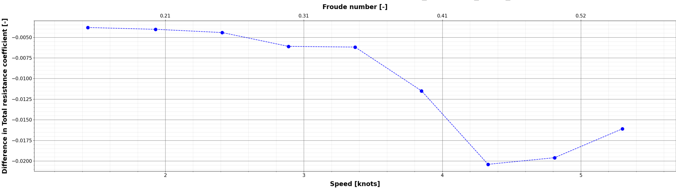
Comparison of Total resistance coefficient : X_{\{i\}} - S60_S768_EFD
