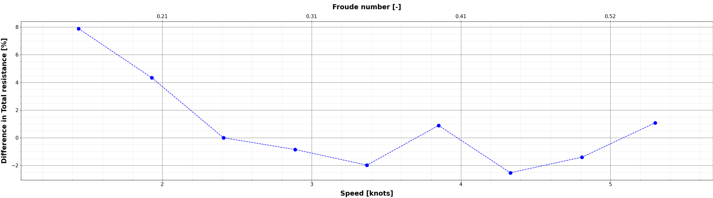
Comparison of Total resistance : (X_{\{i\}} - S60\_S768\_EFD) / S60\_S768\_EFD
