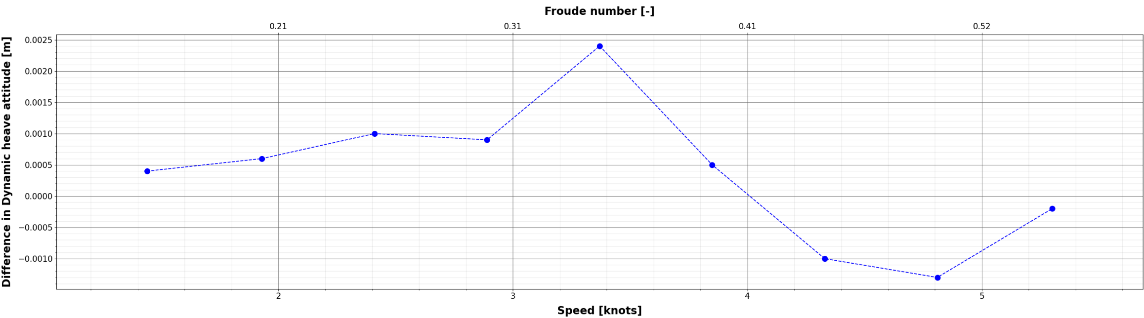
Comparison of Dynamic heave attitude : X_{\{i\}} - S60_S768_EFD
