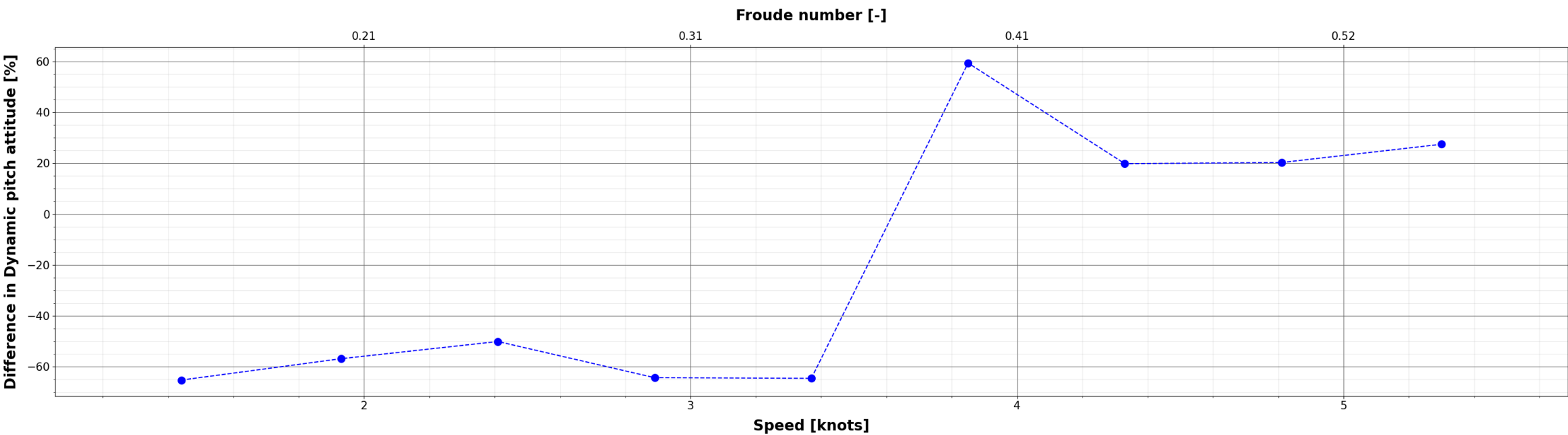
Comparison of Dynamic pitch attitude : (X_{\{i\}} - S60\_S971\_EFD) / S60\_S971\_EFD
