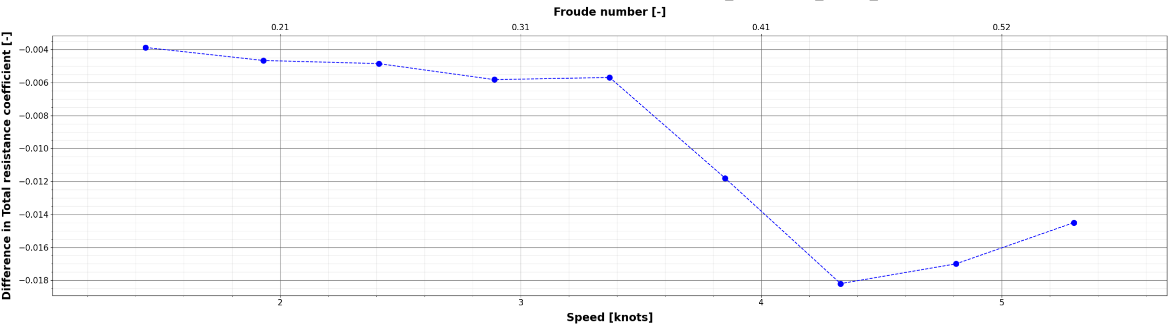
Comparison of Total resistance coefficient : X_{\{i\}} - S60_S971_EFD
