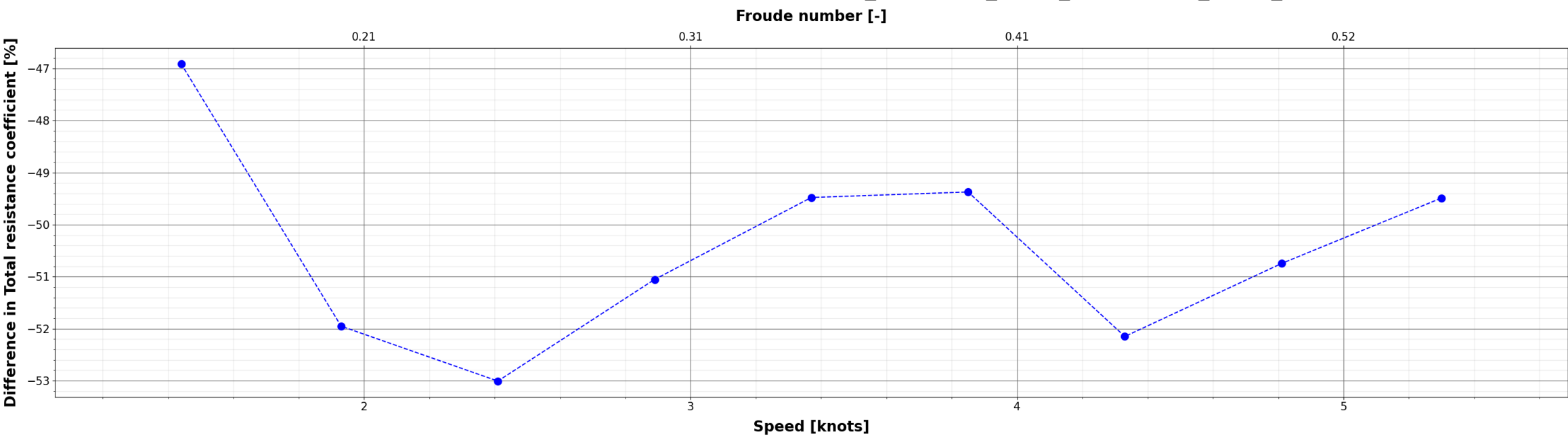
Comparison of Total resistance coefficient : (X_{\{i\}} - S60\_S971\_EFD) / S60\_S971\_EFD
