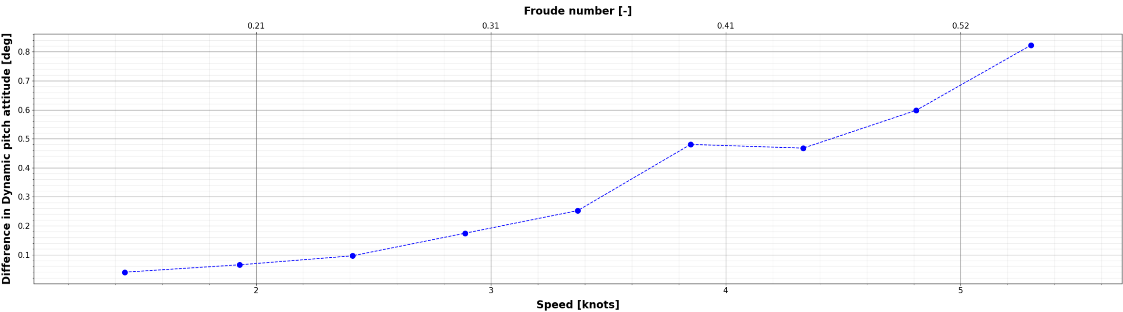
Comparison of Dynamic pitch attitude : X_{\{i\}} - S60_S971_EFD
