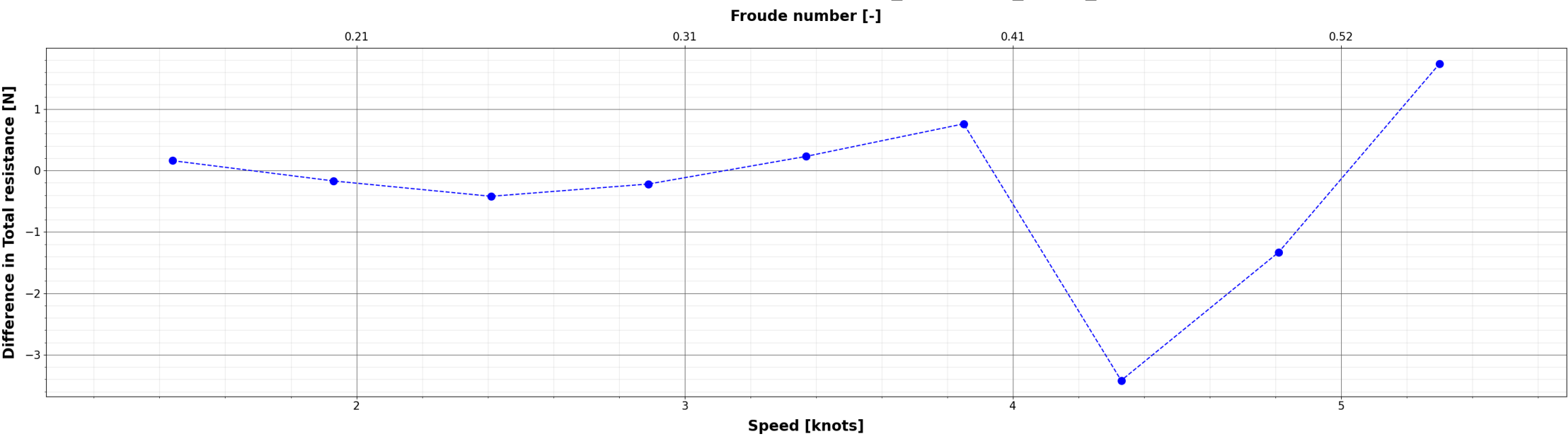
Comparison of Total resistance : X_{\{i\}} - S60_S971_EFD
