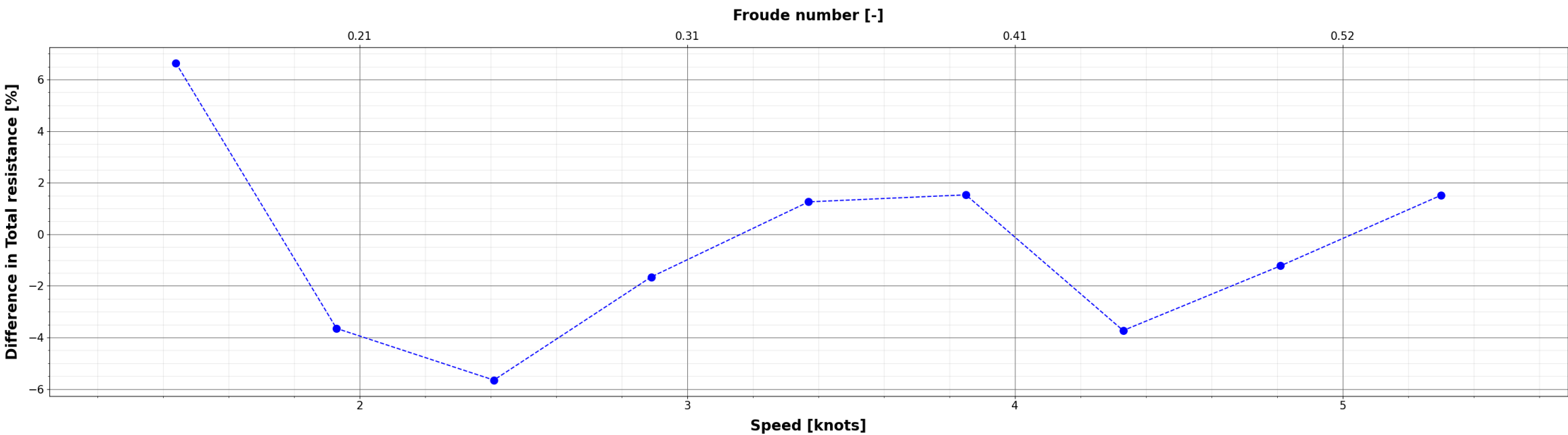
Comparison of Total resistance : (X_{\{i\}} - S60\_S971\_EFD) / S60\_S971\_EFD
