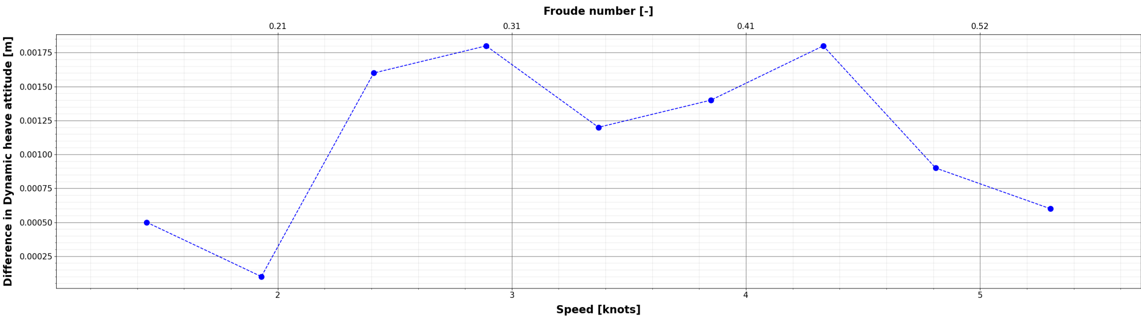
Comparison of Dynamic heave attitude : X_{\{i\}} - S60_S971_EFD
