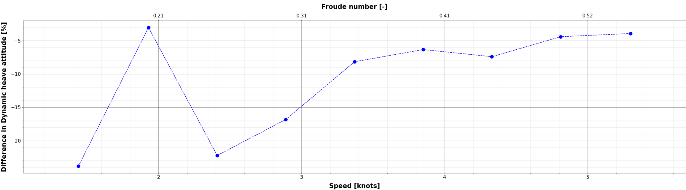
Comparison of Dynamic heave attitude : (X_{\{i\}} - S60\_S971\_EFD) / S60\_S971\_EFD
